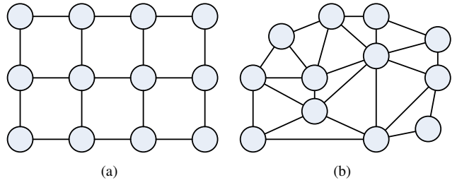
Fig. 1. Generalized thin-membrane model: (a) Regular grid; (b) Irregular grid.
