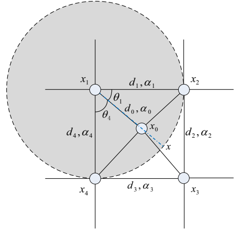
Fig. 2. Illustration of the modified interpolation method
