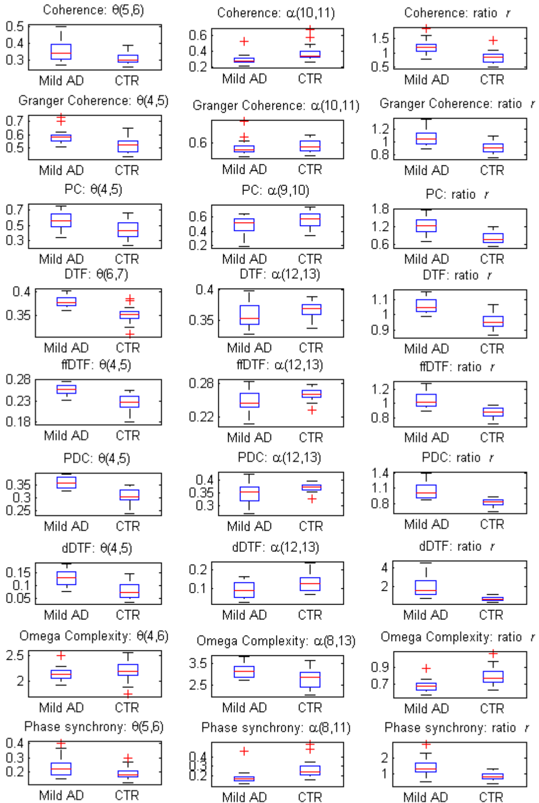
Fig. 2 - Box plots showing the results obtained with the Mild AD data set. Third column shows the results obtained for the ratio. We can observe that box plots are more separated using the ratio than using only \theta or \alpha bands (specific frequency range in Hz on the top of each box plot).
