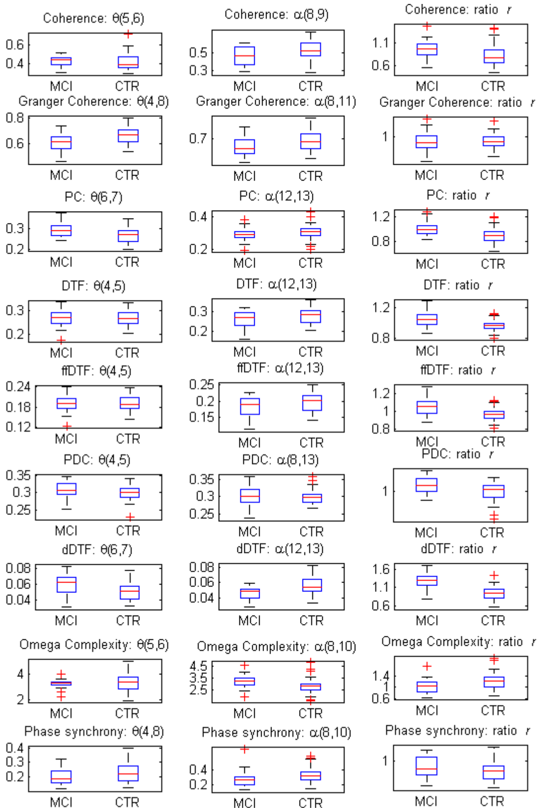
Fig. 1- Box plots showing the results obtained with the MCI data set. Third column shows the results obtained for the ratio. We can observe that box plots are more separated using the ratio than using only \theta or \alpha bands (specific frequency range in Hz on the top of each box plot).
