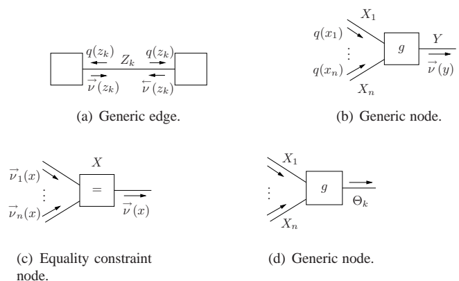
Fig. 2. Variational message passing.
