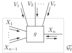
Fig. 3. Structured variational message passing.
