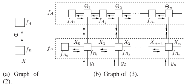
Fig. 1. Factor graphs.
